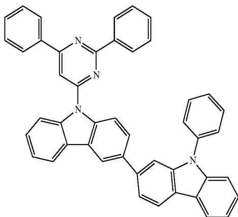
[Chemical formula 10]
